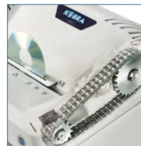
Heavy duty chain drive with steel gears
