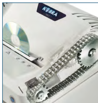
Heavy duty chain drive with steel gears. Security flap.
